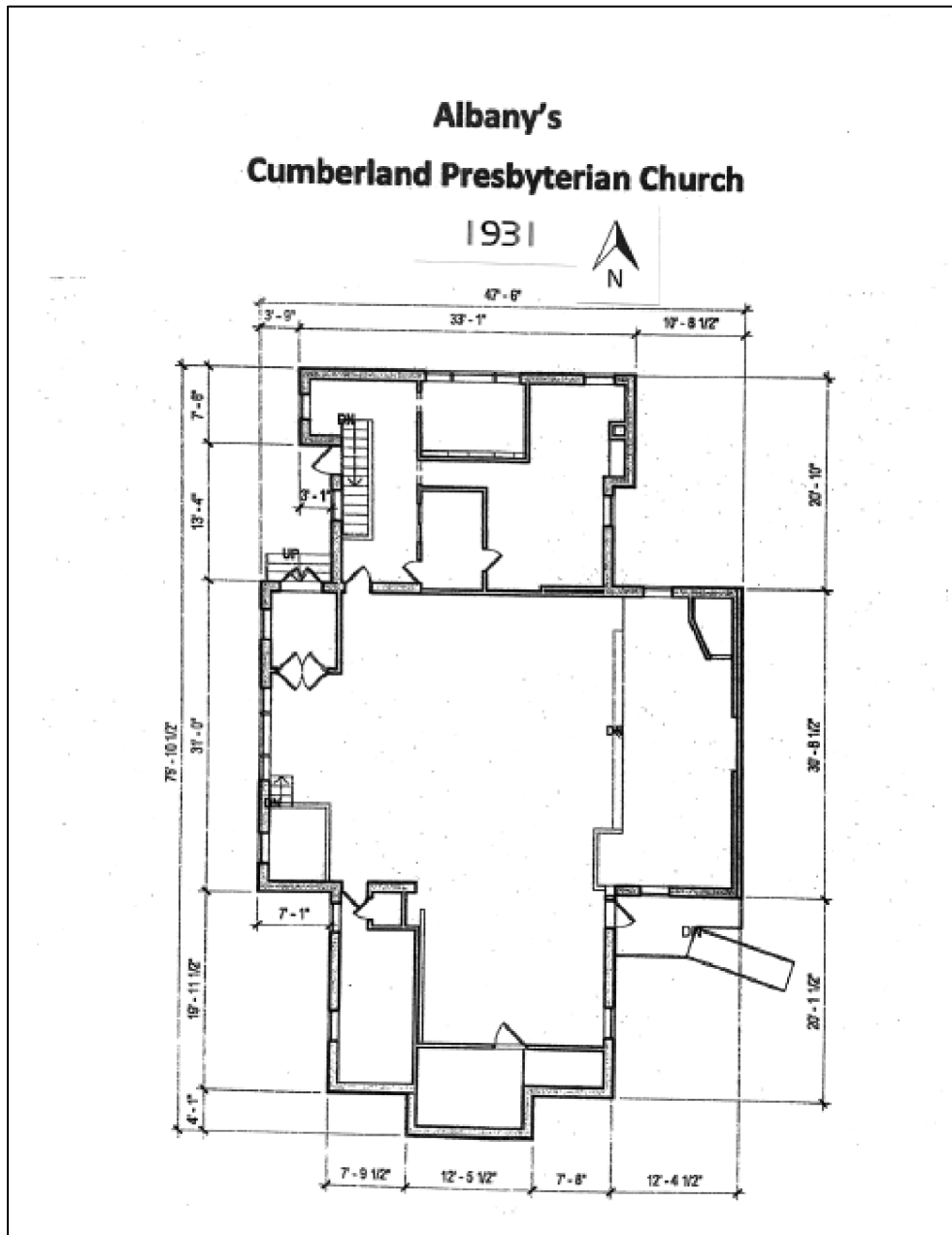
Figure 8: 1931 Floor Plan
