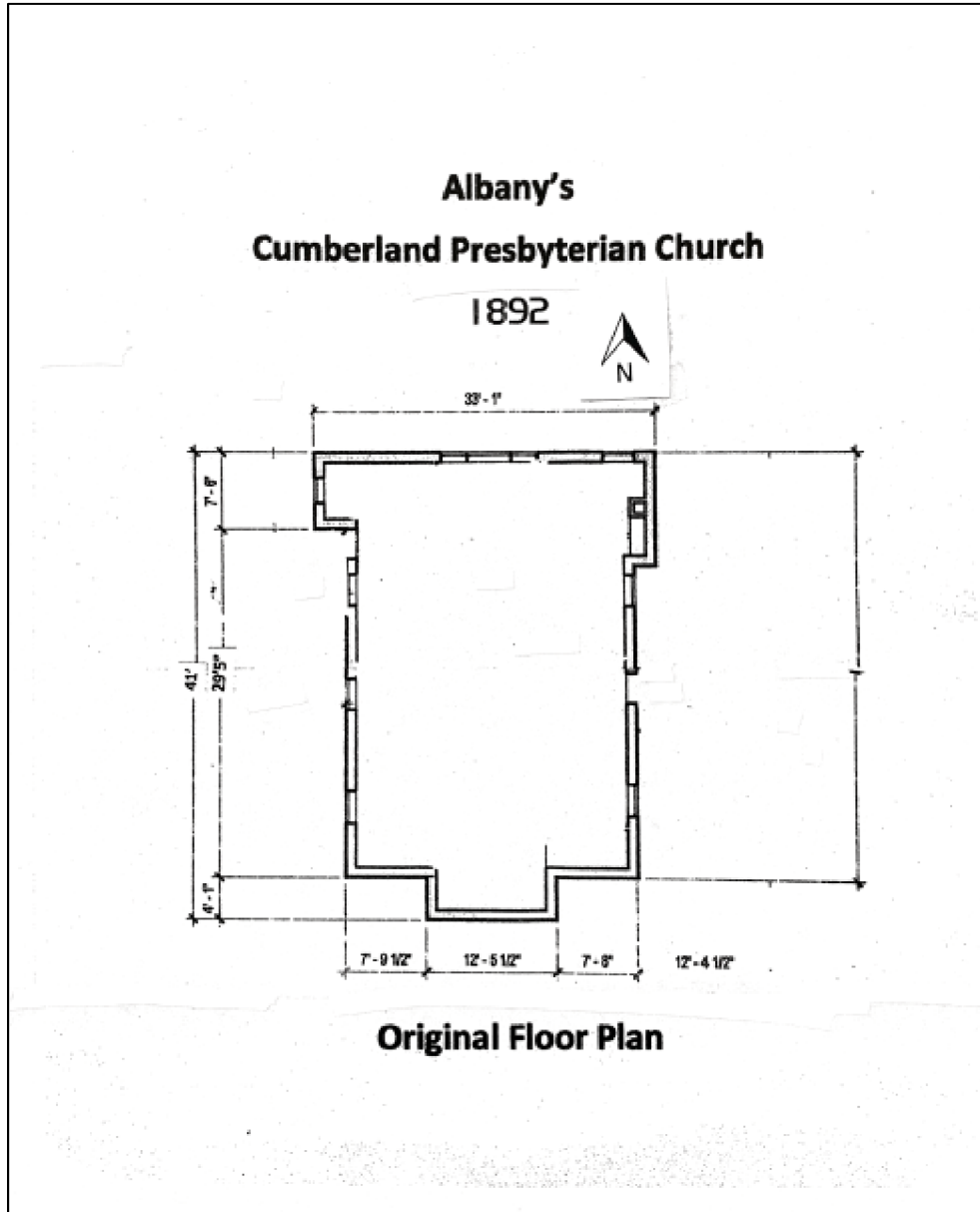
Figure 6: 1892 Floor Plan
