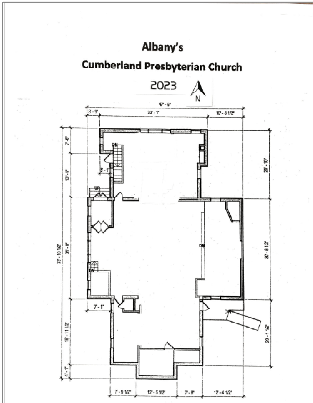
Figure 5: 2023 Floor Plan
